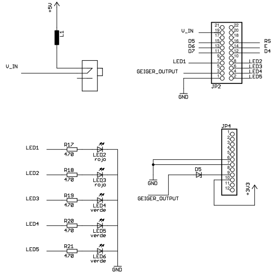
Waspnote connectors
