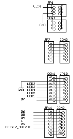
Arduino connectors
